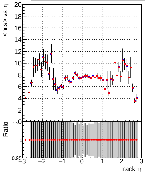
— DQM_V0001_R000000001_Global_mkFit_baseline — DQM_V0001_R000000001_Global_CMSSW_X_Y_Z_RECO
