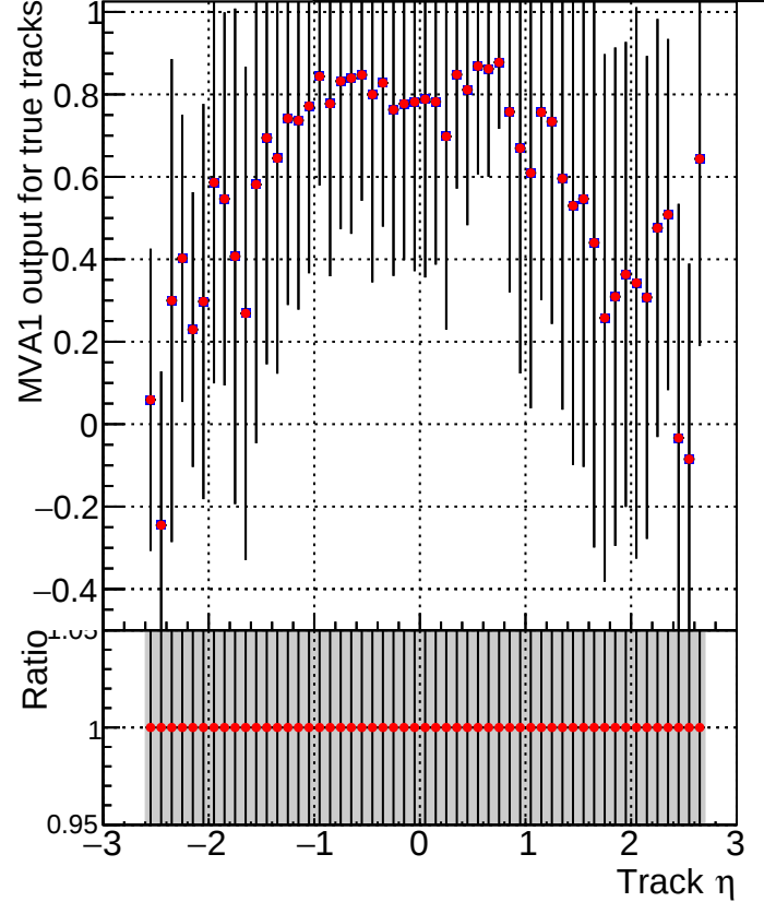
MVA1 of associated tracks (recoToSim) vs. track \eta Legend: ■ DQM_V0001_R000000001_Global_mkFit_baseline ● DQM_V0001_R000000001_Global_CMSSW_X_Y_Z_RECO
