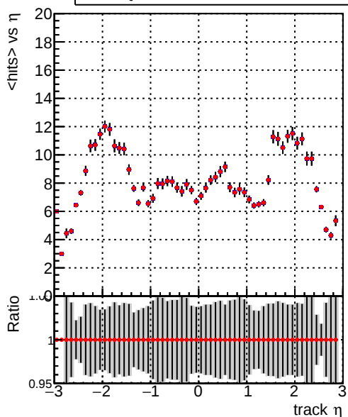
mean hits vs \eta Legend: DQM_V0001_R000000001_Global_mkFit_baseline (blue line), DQM_V0001_R000000001_Global_CMSSW_X_Y_Z_RECO (red line)
