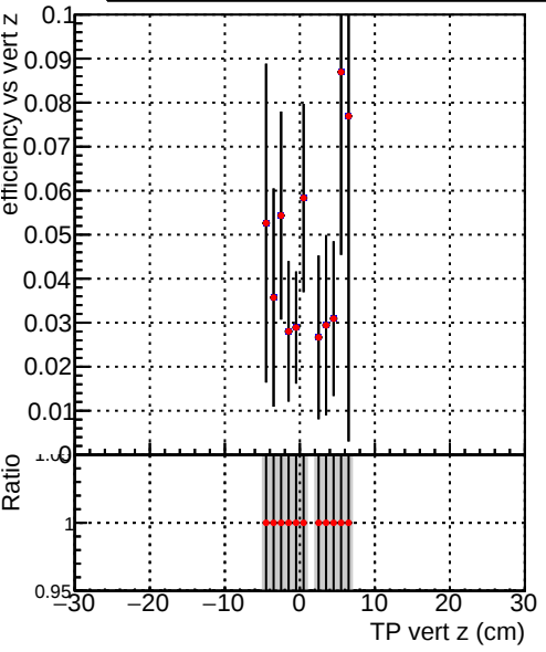
Efficiency vs vert z Legend: DQM_V0001_R000000001_Global_mkFit_baseline DQM_V0001_R000000001_Global_CMSSW_X_Y_Z_RECO
