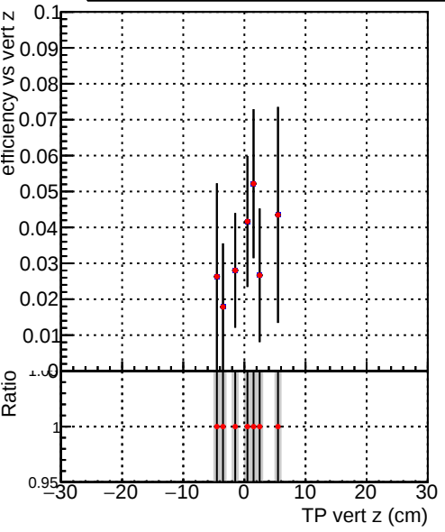
Efficiency vs vertpos Legend: DQM_V0001_R000000001_Global_mkFit_baseline DQM_V0001_R000000001_Global_CMSSW_X_Y_Z_RECO
