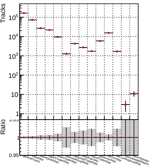
DQM_V0001_R000000001_Global_mkFit_baseline
