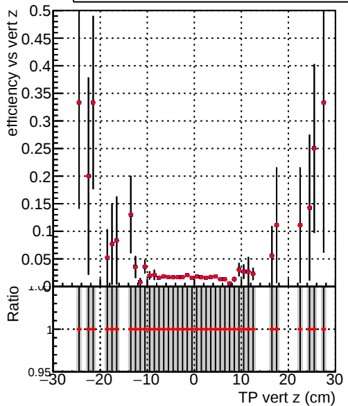
Efficiency vs vert z — DQM_V0001_R000000001_Global_mkFit_baseline — DQM_V0001_R000000001_Global_CMSSW_X_Y_Z_RECO
