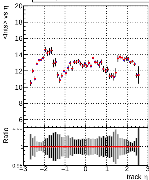
— DQM_V0001_R000000001_Global_mkFit_baseline — DQM_V0001_R000000001_Global_CMSSW_X_Y_Z_RECO
