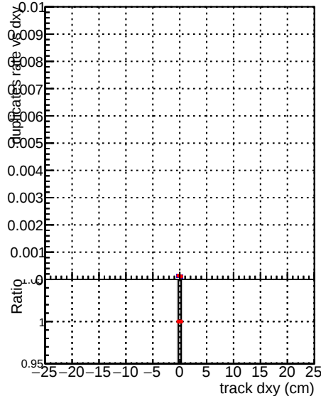
al_mkFit_baseline al_CMSSW_X_Y_Z_REC
