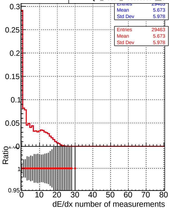
DQM_V0001_R000000001_Global_mkFit_baseline DQM_V0001_R000000001_Global_CMSSW_X_Y_Z_RECO
