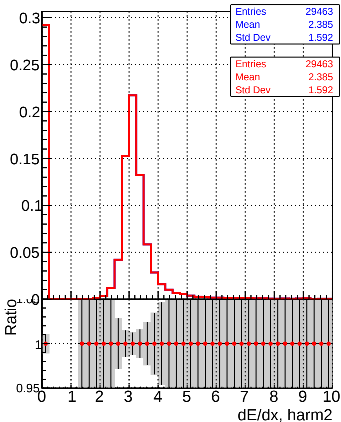
DQM_V0001_R000000001_Global_mkFit_baseline DQM_V0001_R000000001_Global_CMSSW_X_Y_Z_RECO
