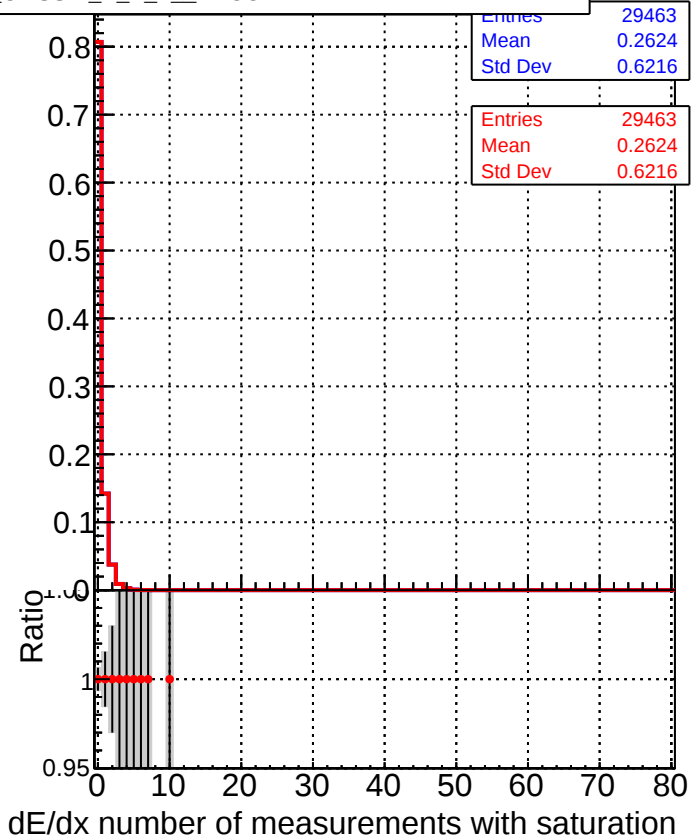
DQM_V0001_R000000001_Global_mkFit_baseline DQM_V0001_R000000001_Global_CMSSW_X_Y_Z_RECO
