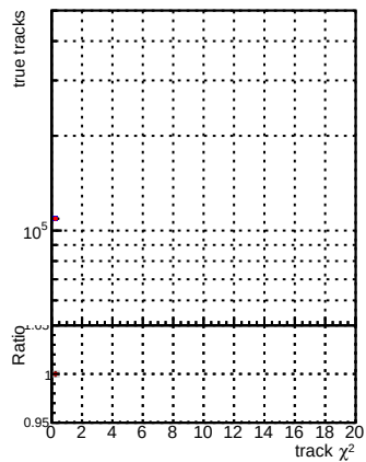
N of reco track vs. \chi^2 for DQM V0001_R000000001 Global CMSSW_X_Y_Z_allINODNN2 DQM V0001_R000000001 Global CMSSW_X_Y_Z_all2
