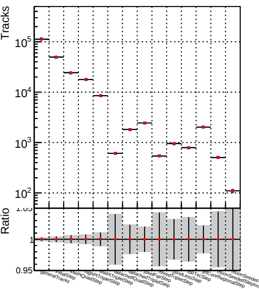
DQM_V0001_R000000001_Global_CMSSW_X_Y_Z_allNODNN2
