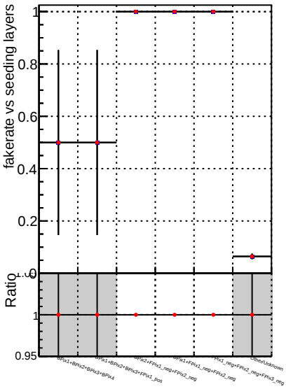
Fake rate vs. DQM_V0001_R000000001 Global CMSSW_X_Y_Z allNODNN2 DQM_V0001_R000000001 Global CMSSW_X_Y_Z all2
