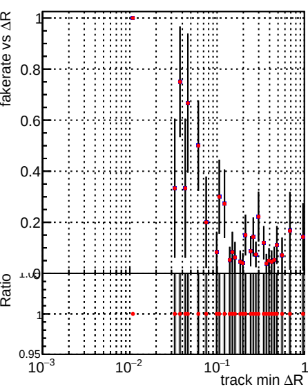
Legend: DQM_V0001_R000000001_Global_CMSSW_X_Y_Z_allNODNN2 (grey shaded), DQM_V0001_R000000001_Global_CMSSW_X_Y_Z_all2 (red line)
