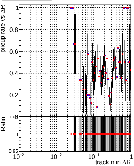
Legend: DQM_V0001_R000000001_Global_CMSSW_X_Y_Z_allNODNN2 (grey shaded), DQM_V0001_R000000001_Global_CMSSW_X_Y_Z_all2 (red line)
