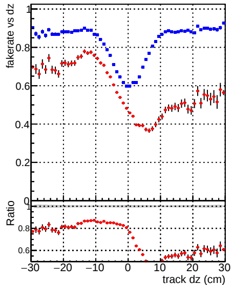
Fake rate vs d DQM_V0001_R000000001 Global CMSSW_X_Y_Z allNODNN2 DQM_V0001_R000000001 Global CMSSW_X_Y_Z all2
