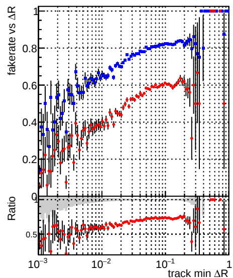
DQM_V0001_R000000001_Global_CMSSW_X_Y_Z_allNODNN2 DQM_V0001_R000000001_Global_CMSSW_X_Y_Z_all2
