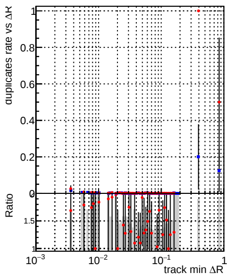
DQM_V0001_R000000001_Global_CMSSW_X_Y_Z_allNODNN2 DQM_V0001_R000000001_Global_CMSSW_X_Y_Z_all2
