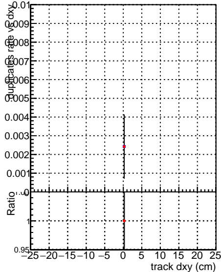
■ DQM_V0001_R000000001_Global_CMSSW_X_Y_Z_allNODNN2 ■ DQM_V0001_R000000001_Global_CMSSW_X_Y_Z_all2
