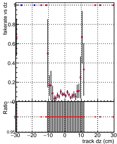
■ DQM_V0001_R000000001_Global_CMSSW_X_Y_Z_allNODNN2 ■ DQM_V0001_R000000001_Global_CMSSW_X_Y_Z_all2
