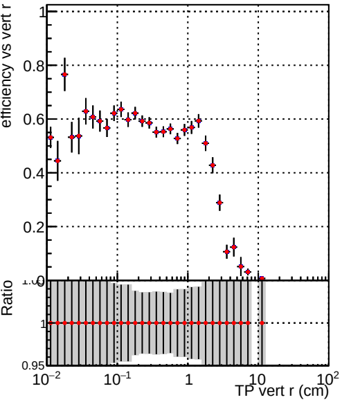
Efficiency vs vertpos Legend: DQM_V0001_R000000001_Global_CMSSW_X_Y_Z_allNODNN2 DQM_V0001_R000000001_Global_CMSSW_X_Y_Z_all2
