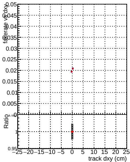
Global CMSSW_X_Y_Z allNODNN2 Fake rate vs d DQM_V0001_R0000000001 DQM_V0001_R0000000001 DQM_V0001_R0000000001 Duplicates Rate vs Dxy DQM_V0001_R0000000001 DQM_V0001_R0000000001 DQM_V0001_R0000000001 Pileup rate vs dxy DQM_V0001_R0000000001 DQM_V0001_R0000000001 DQM_V0001_R0000000001
