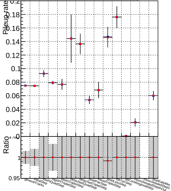
DQM_V0001_R000000001_Global_CMSSW_X_Y_Z_allNODNN DQM_V0001_R000000001_Global_CMSSW_X_Y_Z_all
