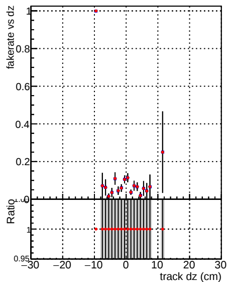
Fake rate vs dz —●— DQM_V0001_R0000000001 Global CMSSW_X_Y_Z_allINODNN —●— DQM_V0001_R0000000001 Global CMSSW_X_Y_Z_all
