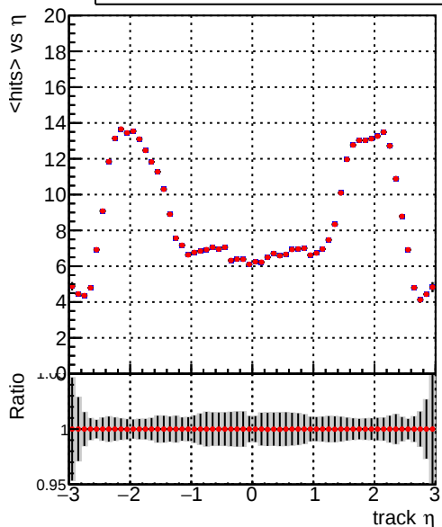
mean hits — DQM_V0001_R000000001_Global_CMSSW_X_Y_Z_allNODNN — DQM_V0001_R000000001_Global_CMSSW_X_Y_Z_all
