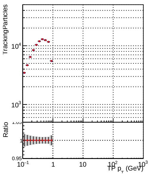
Legend: - \text{DQM\_V0001\_R000000001\_Global\_CMSSW\_X\_Y\_Z\_allNODNN} (blue line) - \text{DQM\_V0001\_R000000001\_Global\_CMSSW\_X\_Y\_Z\_all} (red line)
