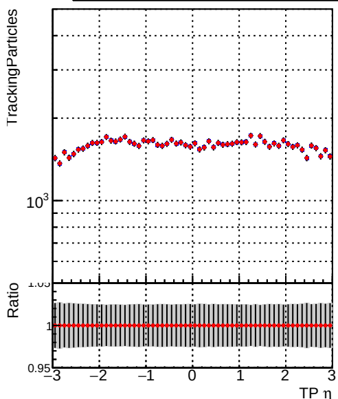
Legend: - \text{DQM\_V0001\_R000000001\_Global\_CMSSW\_X\_Y\_Z\_allNODNN} (blue line) - \text{DQM\_V0001\_R000000001\_Global\_CMSSW\_X\_Y\_Z\_all} (red line)
