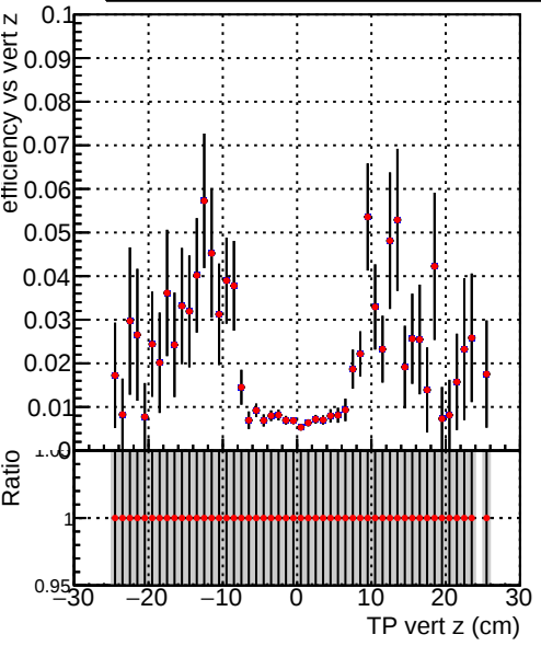
Efficiency vs vert z Legend: DQM_V0001_R000000001_Global_CMSSW_X_Y_Z_allINODNN DQM_V0001_R000000001_Global_CMSSW_X_Y_Z_all
