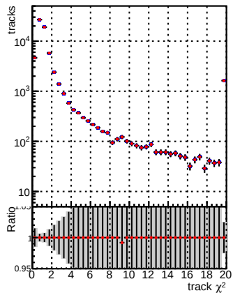
N of reco track vs. \chi^2 for DQM_V0001_R000000001_Global_CMSSW_X_Y_Z_allINODNN and DQM_V0001_R000000001_Global_CMSSW_X_Y_Z_all
