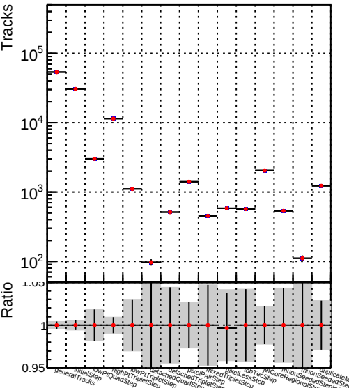
DQM_V0001_R000000001__Global__CMSSW_X_Y_Z__allNODNN
