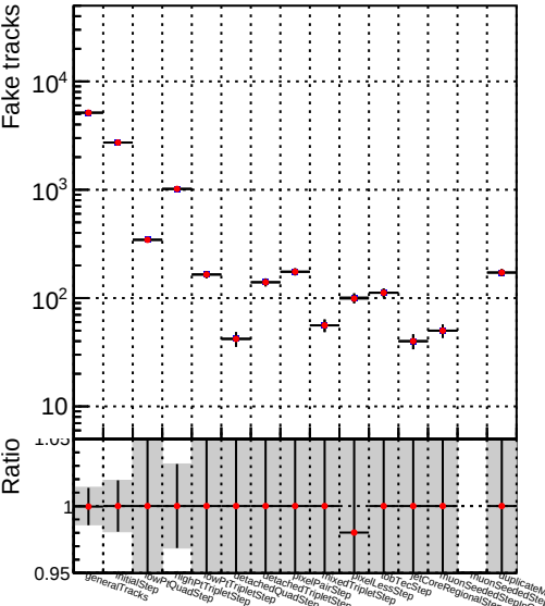
Number ● DQM_V0001_R000000001_Global_CMSSW_X_Y_Z_all
