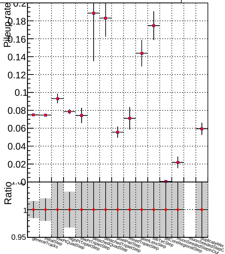
DQM_V0001_R000000001_Global_CMSSW_X_Y_Z_allNODNN DQM_V0001_R000000001_Global_CMSSW_X_Y_Z_all
