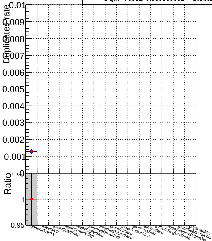
DQM_V0001_R000000001_Global_CMSSW_X_Y_Z_allNODNN DQM_V0001_R000000001_Global_CMSSW_X_Y_Z_all
