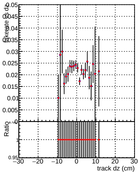
Fake rate vs dz —●— DQM_V0001_R0000000001_Global_CMSSW_X_Y_Z_allNODNN —●— DQM_V0001_R0000000001_Global_CMSSW_X_Y_Z_all
