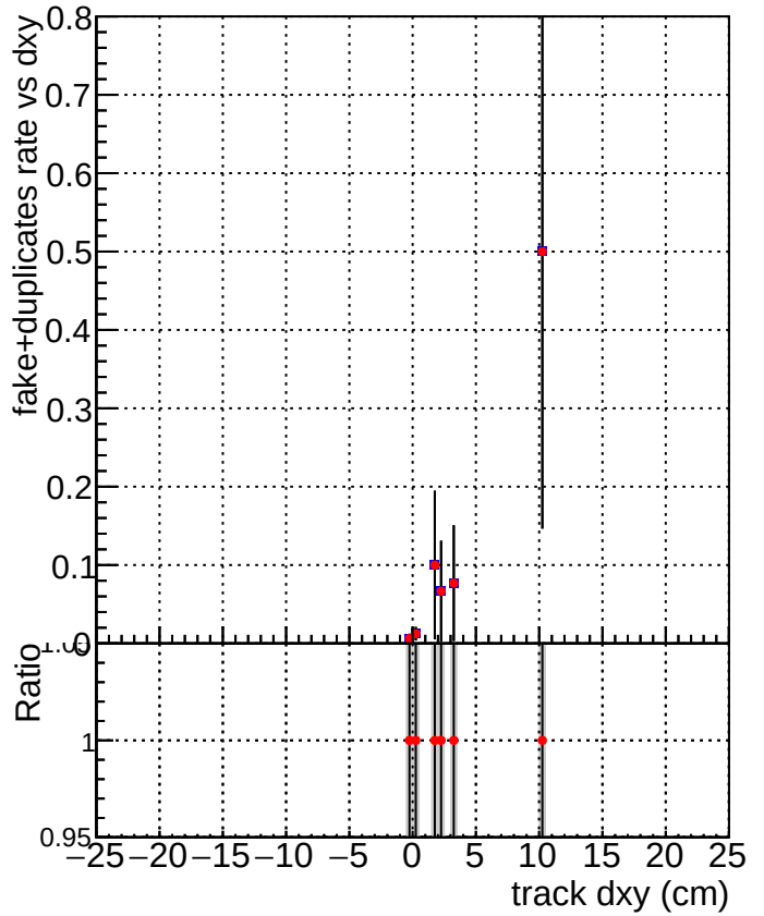
DQM_V0001_R000000001_Global_CMSSW_X_Y_Z_allINODNN DQM_V0001_R000000001_Global_CMSSW_X_Y_Z_all
