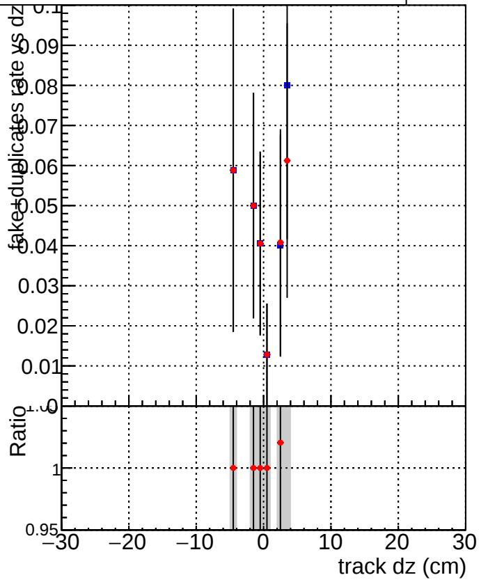
DQM_V0001_R000000001_Global_CMSSW_X_Y_Z_allINODNN DQM_V0001_R000000001_Global_CMSSW_X_Y_Z_all
