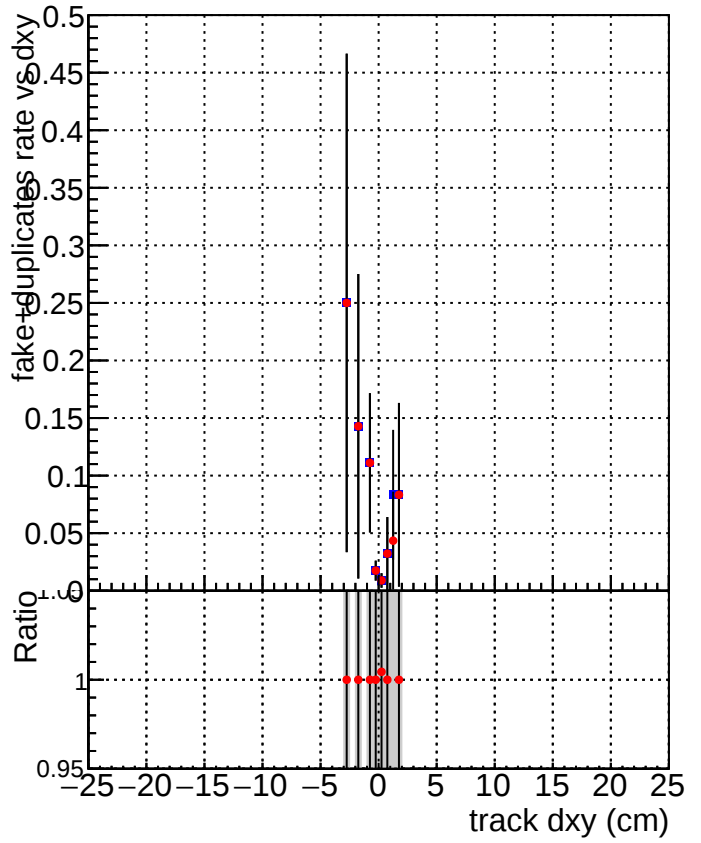
DQM_V0001_R000000001_Global_CMSSW_X_Y_Z_allINODNN DQM_V0001_R000000001_Global_CMSSW_X_Y_Z_all
