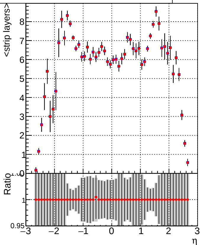
Legend: DQM_V0001_R000000001_Global_CMSSW_X_Y_Z_allINODNN DQM_V0001_R000000001_Global_CMSSW_X_Y_Z_all
