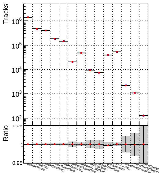
DQM_V0001_R000000001__Global__CMSSW_X_Y_Z__allNODNN
