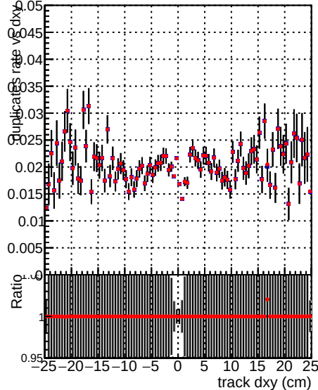
Global CMSSW_X_Y_Z all all DQM_V0001_R0000000001 Global CMSSW_X_Y_Z all
