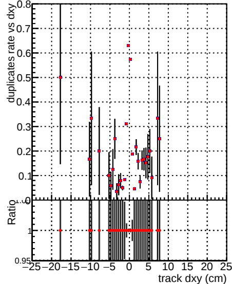
—●— DQM_V0001_R0000000001 Global CMSSW_X_Y_Z alINODNN —●— DQM_V0001_R0000000001 Global CMSSW_X_Y_Z all
