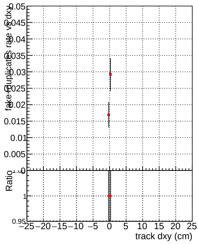
DQM_V0001_R000000001_Global_CMSSW_X_Y_Z_allINODNN
