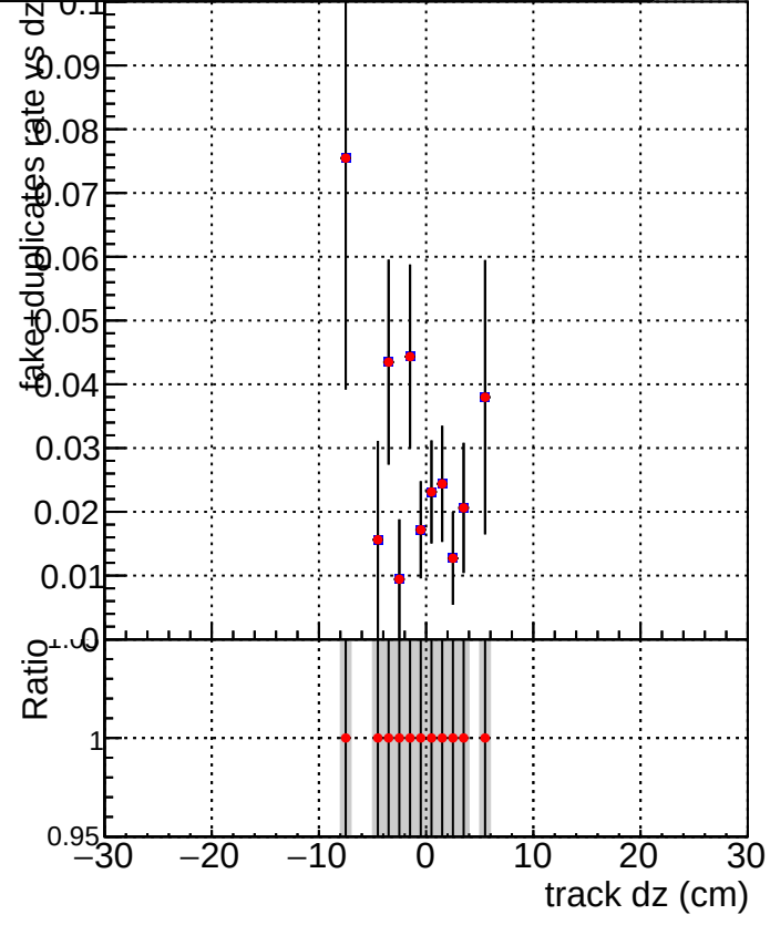
DQM_V0001_R000000001_Global_CMSSW_X_Y_Z_allINODNN
