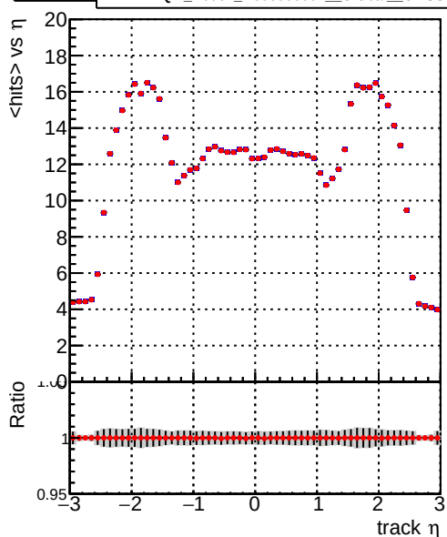
— DQM_V0001_R000000001_Global_CMSSW_X_Y_Z_allNODNN — DQM_V0001_R000000001_Global_CMSSW_X_Y_Z_all
