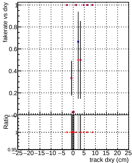
—●— DQM_V0001_R0000000001 Global CMSSW X Y Z all NODNN —●— DQM_V0001_R0000000001 Global CMSSW X Y Z all
