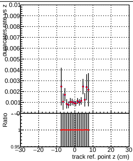
—•— DQM_V0001_R000000001_Global_CMSSW_X_Y_Z_allINODNN —•— DQM_V0001_R000000001_Global_CMSSW_X_Y_Z_all
