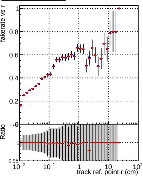
—•— DQM_V0001_R000000001_Global_CMSSW_X_Y_Z_allINODNN —•— DQM_V0001_R000000001_Global_CMSSW_X_Y_Z_all
