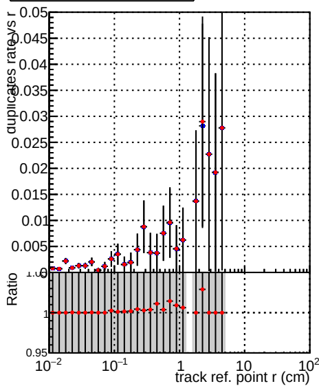
—•— DQM_V0001_R000000001_Global_CMSSW_X_Y_Z_allINODNN —•— DQM_V0001_R000000001_Global_CMSSW_X_Y_Z_all
