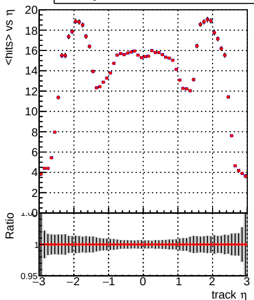
mean hits — DQM_V0001_R000000001_Global_CMSSW_X_Y_Z_allNODNN — DQM_V0001_R000000001_Global_CMSSW_X_Y_Z_all
