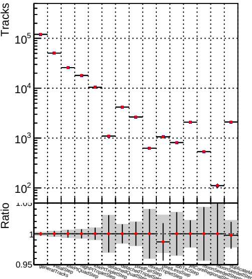
DQM_V0001_R000000001__Global__CMSSW_X_Y_Z__allNODNN
