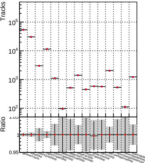
DQM_V0001_R000000001__Global__CMSSW_X_Y_Z__allNODNN
