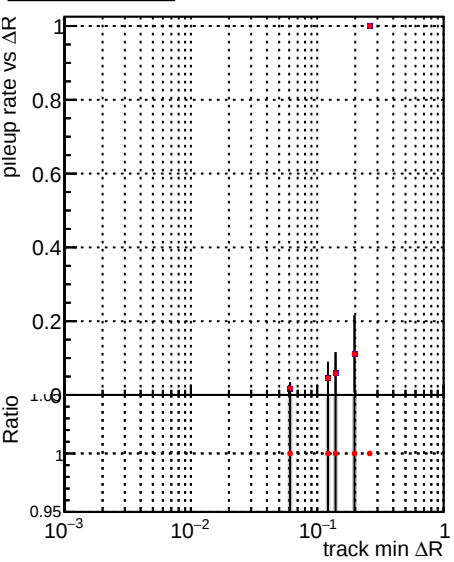
Legend: - \Delta R(\text{track}, \text{jet}) - \Delta R(\text{track}, \text{jet})
