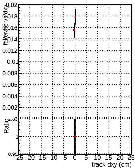
—●— DQM_V0001_R0000000001 Global CMSSW_X_Y_Z_allNODNN —●— DQM_V0001_R0000000001 Global CMSSW_X_Y_Z_all
