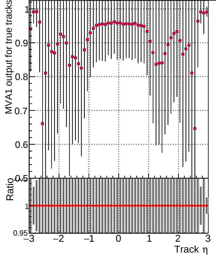
MVA1 of associated tracks (recoToSim) vs. track \eta Legend: ■ DQM_V0001_R000000001_Global_CMSSW_X_Y_Z_allINODNN ● DQM_V0001_R000000001_Global_CMSSW_X_Y_Z_all
