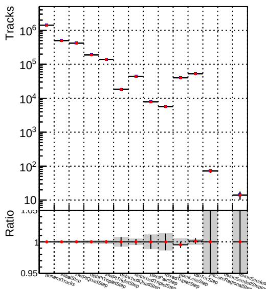
DQM_V0001_R000000001_Global_CMSSW_X_Y_Z_allNODNN
