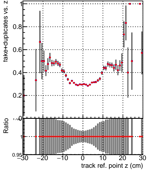
■ DQM_V0001_R000000001_Global_CMSSW_X_Y_Z_allNODNN ◆ DQM_V0001_R000000001_Global_CMSSW_X_Y_Z_all
