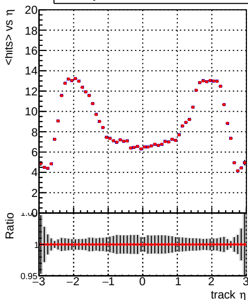
mean hits vs \eta Legend: DQM_V0001_R000000001_Global_CMSSW_X_Y_Z_allNODNN (blue line), DQM_V0001_R000000001_Global_CMSSW_X_Y_Z_all (red line)
