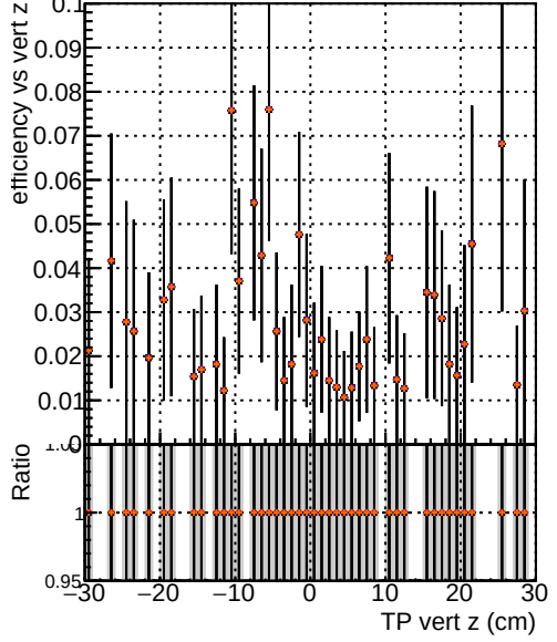
Efficiency vs vert z Legend Series Model Global CMSSW X Y Z all all75 all175 Blue line DQM_V0001 R0000000001 Global CMSSW X Y Z all all75 all175 Red line DQM_V0001 R0000000001 Global CMSSW X Y Z all all75 all175 Black line DQM_V0001 R0000000001 Global CMSSW X Y Z all all75 all175 Orange line DQM_V0001 R0000000001 Global CMSSW X Y Z all all75 all175
