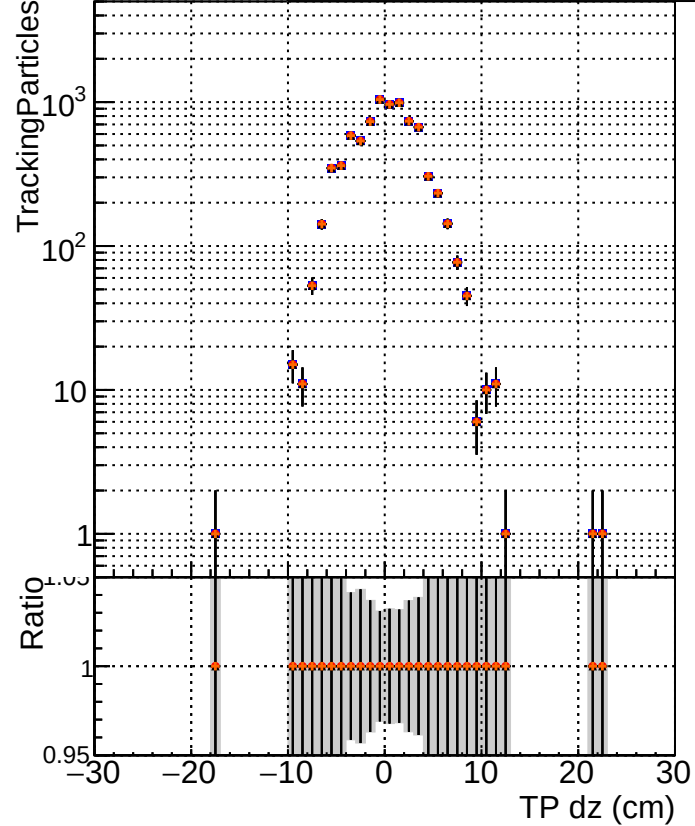
N of simulated track Legend Legend Legend Legend ■ DQM_V0001_R000000001 Global CMSSW_X_Y_Z allNODNN2 ● DQM_V0001_R000000001 Global CMSSW_X_Y_Z all2 ▲ DQM_V0001_R000000001 Global CMSSW_X_Y_Z all75 ◆ DQM_V0001_R000000001 Global CMSSW_X_Y_Z all7
