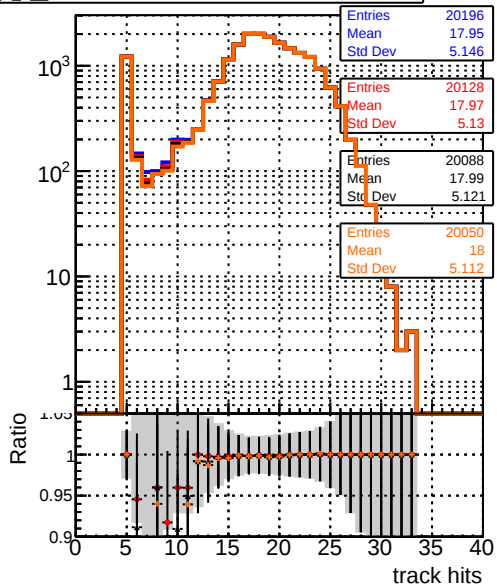
mean hits > \eta DQM_V0001_R000000001_Global_CMSSW_X_Y_Z_allNODBN2 DQM_V0001_R000000001_Global_CMSSW_X_Y_Z_all2 DQM_V0001_R000000001_Global_CMSSW_X_Y_Z_all75 DQM_V0001_R000000001_Global_CMSSW_X_Y_Z_all7
